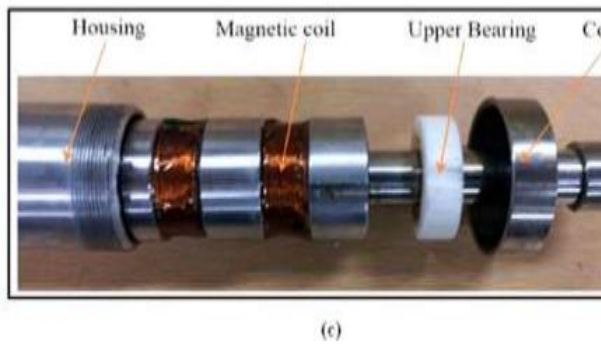
FIG. 3. MR model damper: (a) Setup, (b) Magnetic core damper and (c) Practical magnetic core MR model.
