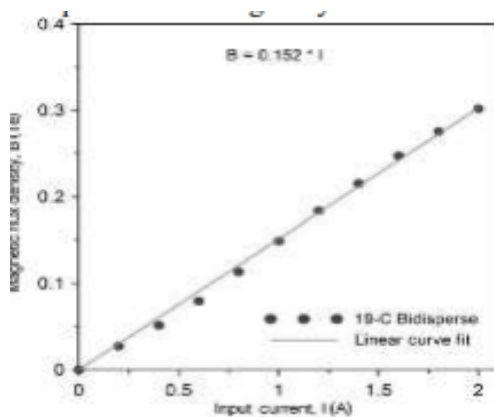
Figure 2. The magnet flux density adjustment (B, T) depending on the input current at the distance between the viscometer's parallel discs. Figure 1. shows the input current and magnetic flux density
