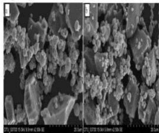
Fig. 1. Microgram of (a) Monodisperse abrasive magnetic (sample 1); (b) Attractive abrasive bidis perse (test 3)
